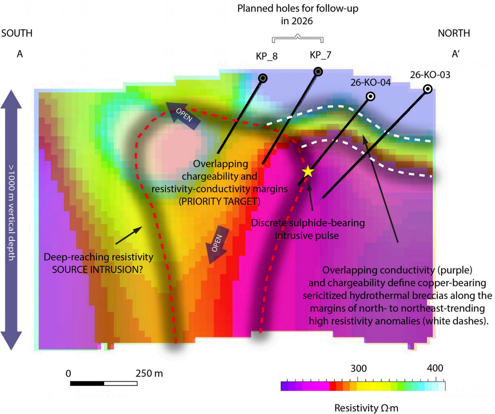
BERTHA NORTH - Oblique Longitudinal Section Looking West
